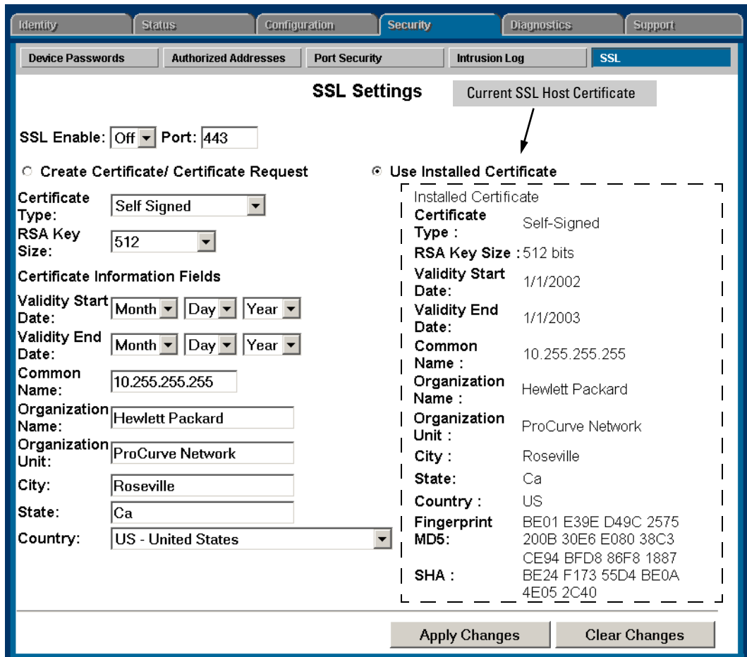
Figure 8-6. Web browser Interface showing current SSL Host Certificate
